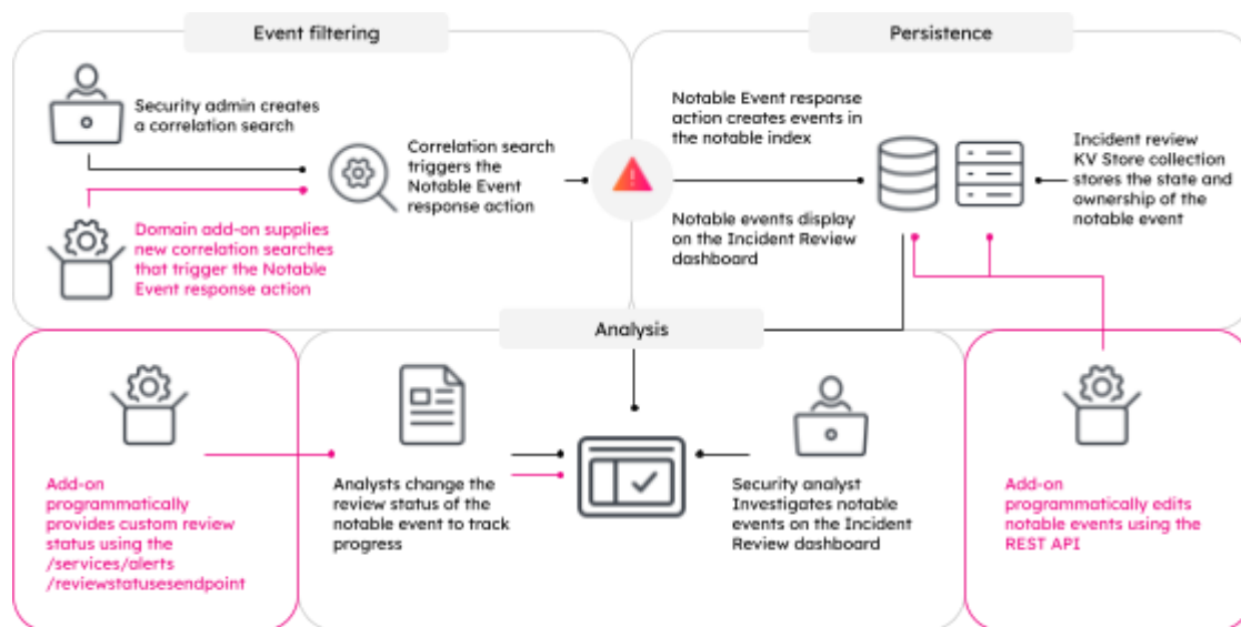
Flow of a Notable Event created from events in Splunk into the Incident Review dashboard.
